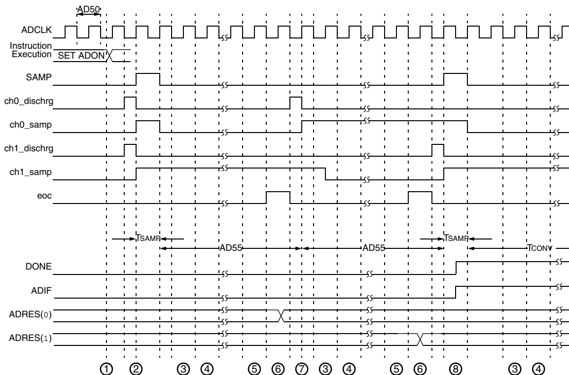
FIGURE 23-26: 10-BIT HIGH-SPEED A/D CONVERSION TIMING CHARACTERISTICS (CHPS = 01, SIMSAM = 0, ASAM = 1, SSRC = 111, SAMC = 00001)
