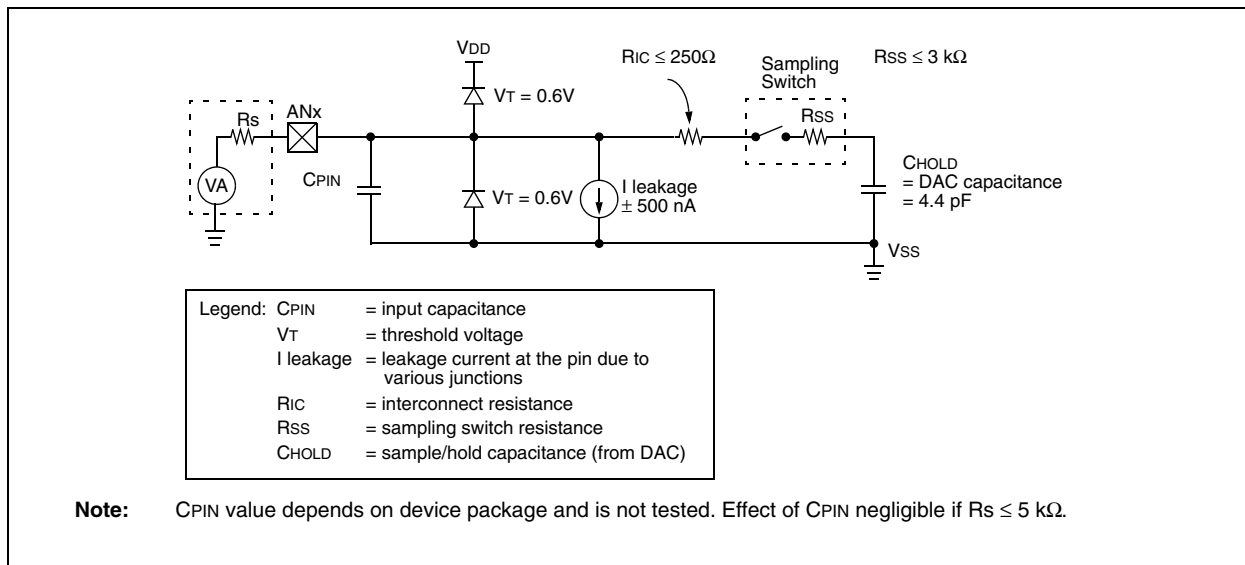
FIGURE 19-2: A/D CONVERTER ANALOG INPUT MODEL
