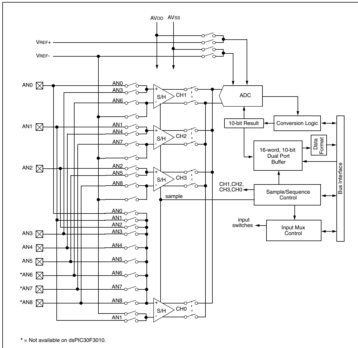
FIGURE 19-1: 10-BIT HIGH SPEED A/D FUNCTIONAL BLOCK DIAGRAM
