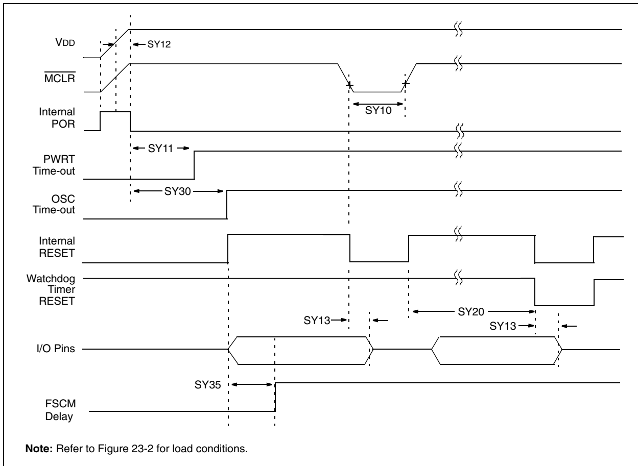
FIGURE 23-5: RESET, WATCHDOG TIMER, OSCILLATOR START-UP TIMER AND POWER-UP TIMER TIMING CHARACTERISTICS
