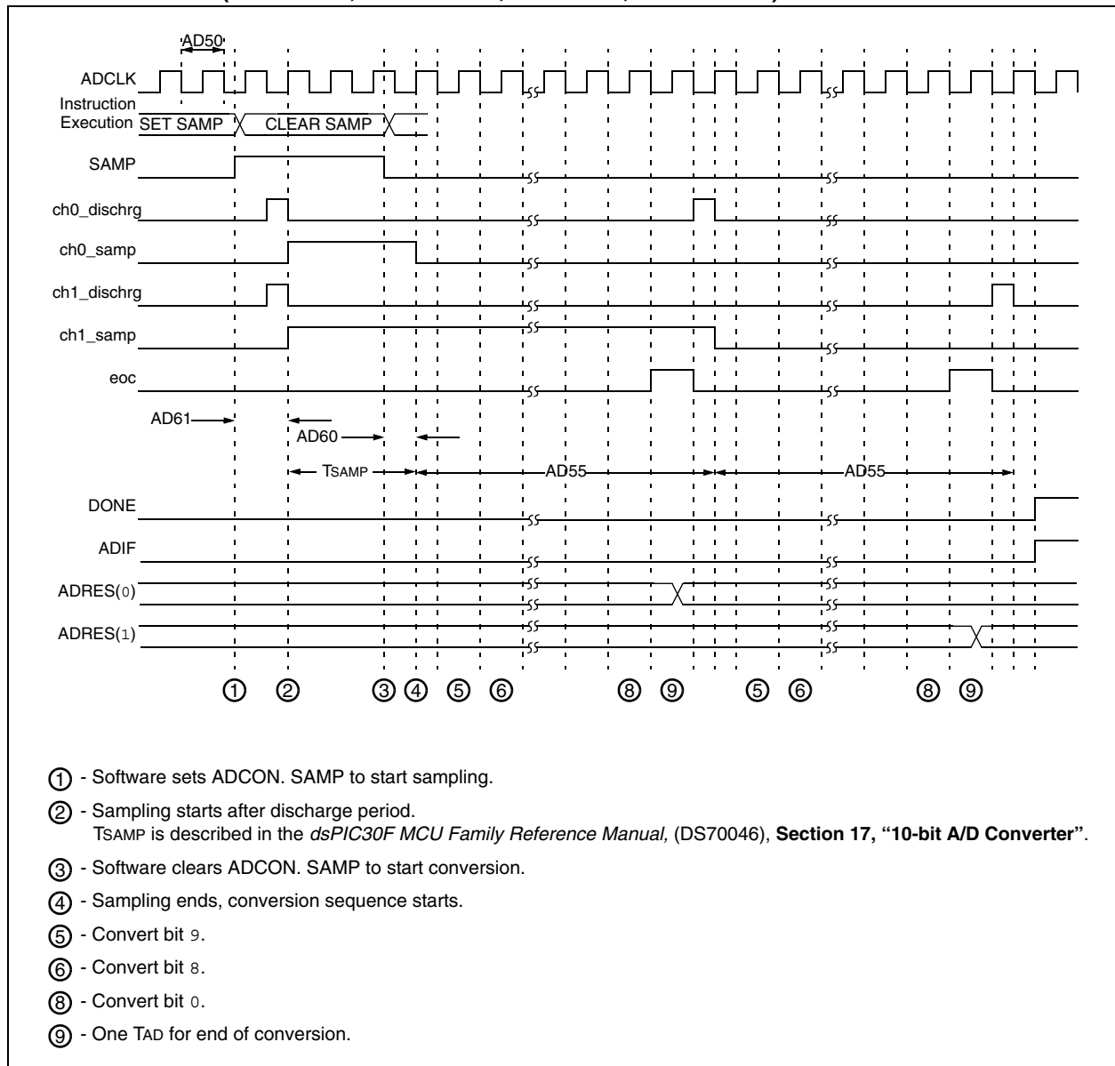
FIGURE 23-25: 10-BIT HIGH-SPEED A/D CONVERSION TIMING CHARACTERISTICS (CHPS = 01, SIMSAM = 0, ASAM = 0, SSRC = 000)
