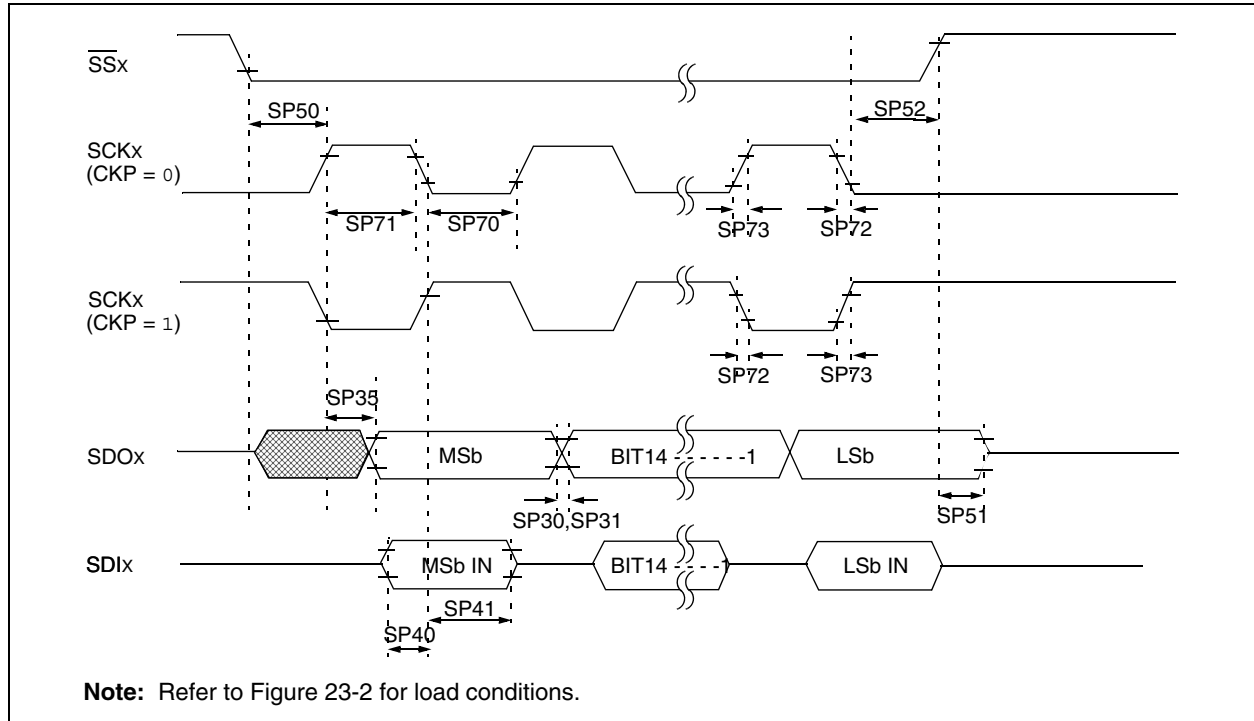
FIGURE 23-18: SPI™ MODULE SLAVE MODE (CKE = 0) TIMING CHARACTERISTICS
