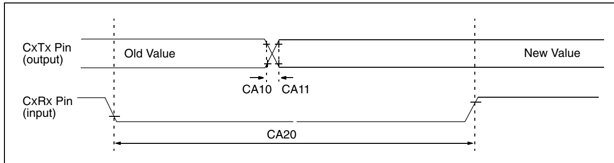
FIGURE 23-24: CAN MODULE I/O TIMING CHARACTERISTICS
