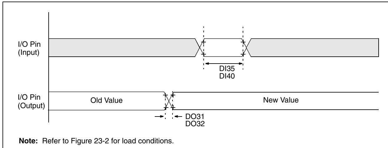
FIGURE 23-4: CLKOUT AND I/O TIMING CHARACTERISTICS
